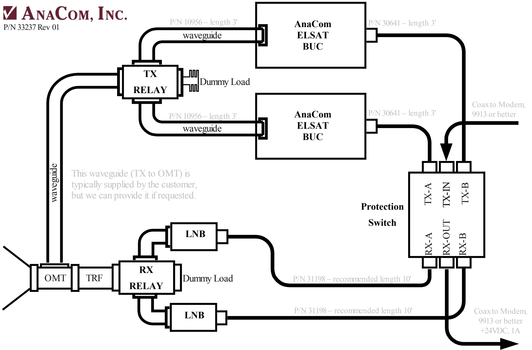
1+1 Redundant Protection Switch for two ELSAT BUCs and LNB protection. This diagram shows RF/IF connections only, the control cables (PS to BUCs & PX to Relays) are not shown
